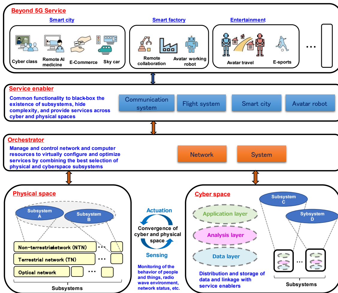
Figure 6.6-5 Beyond 5G architecture application to resilience 13
