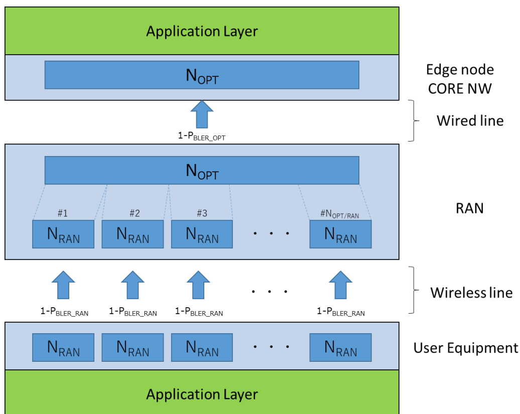
Figure 5.3-5 An examination model for End-to-End transmission
