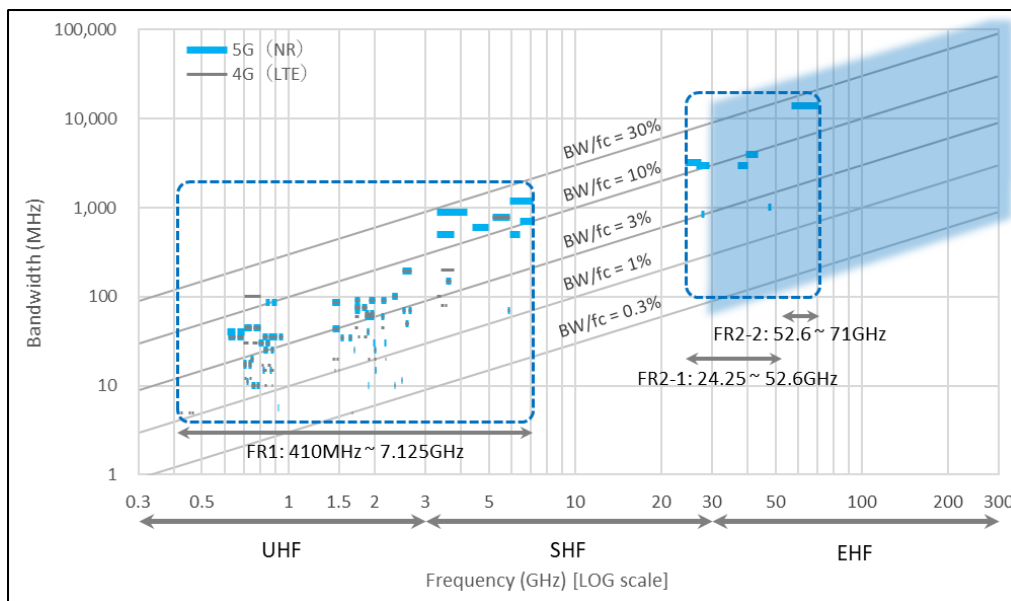
Figure 6.1-5 Frequency bands defined for 4G and 5G (3GPP specifications [1] [2] [3] [4]) and expansion to EHF band
