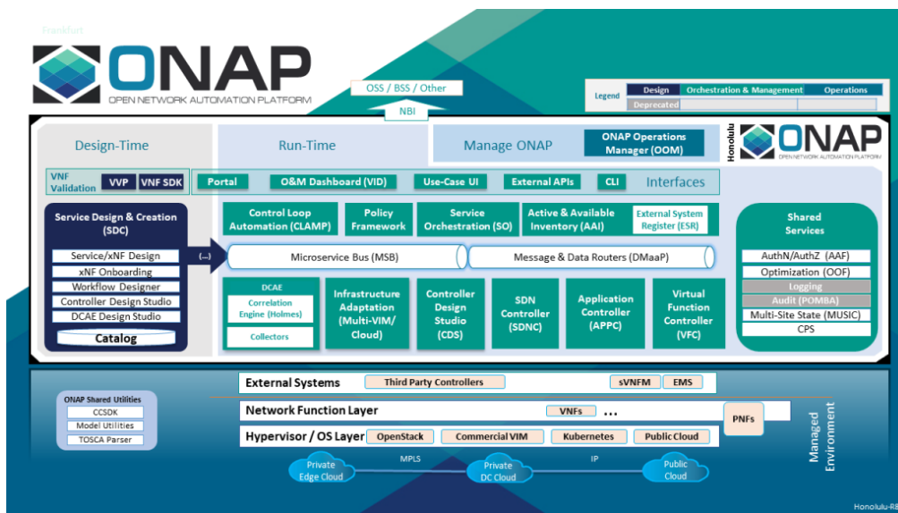
Figure 6.6-2 Overall architecture of ONAP [15]
