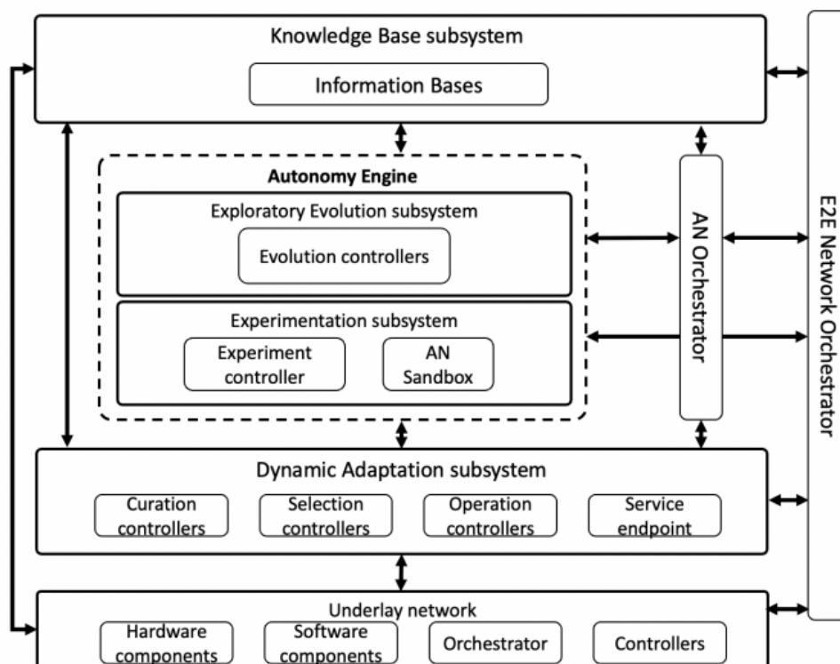
Figure 6.6-3 Examples of control architectures for autonomous networks [18]
