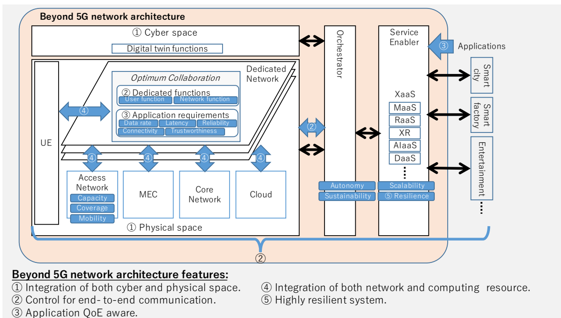
Figure 6.6-1 Beyond 5G network architecture
