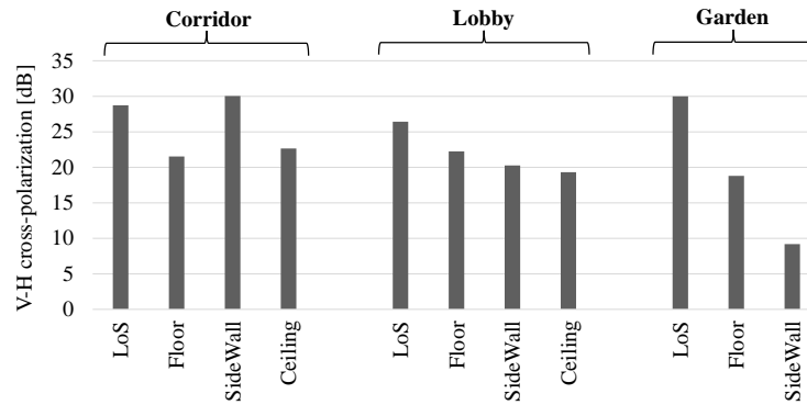
Figure 6.3-15 Effect of indoor structures on cross-polarization
