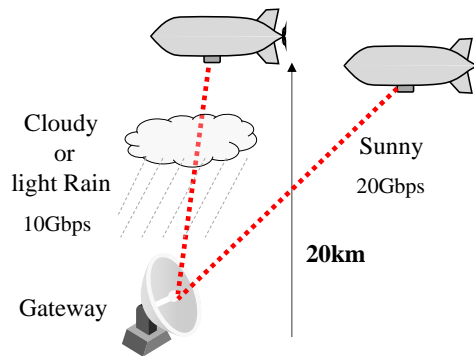
Figure 6.3-12 Concept of ground to NTN communication using 100GHz band
