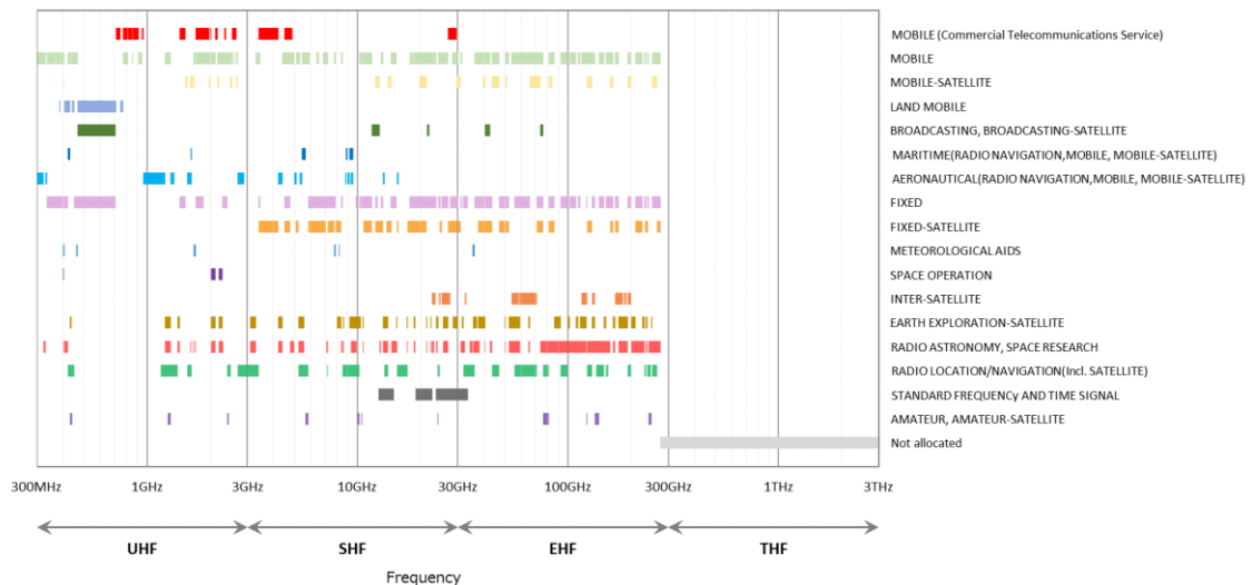
Figure 6.3-2 Frequency assignments in Japan [5]
