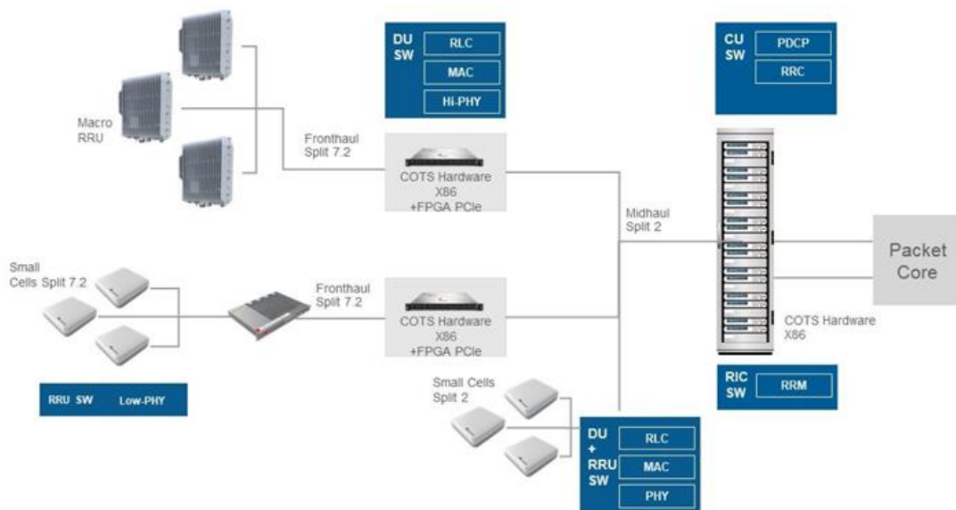
図 2-12Next-Generation Operations Support Systems の構成
