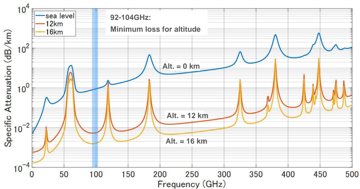
Figure 6.1-14 Propagation losses due to atmospheric gases and related effects [2]
