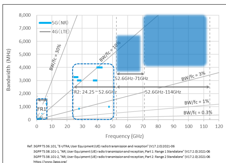
Figure 6.1-5 Frequency bands defined for 4G and 5G in the 3GPP specifications [1] [2] [3]
